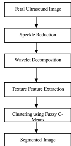
Fig. 1. Block diagram of the proposed segmentation algorithm
