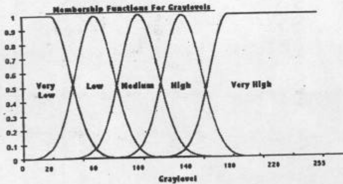
Figure 1. Fuzzy membership functions for the 9 graylevels used in both algorithms
